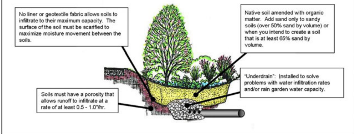
Fig. 12 Rain garden design with a mixed soil medium and an underdrain Graphic by Joe Boggs modified from DER, 2002
